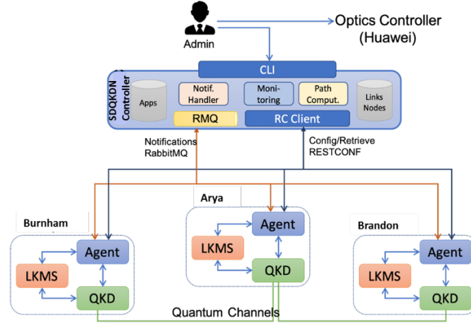
Figure 2: SW structure of the network. A SDN Controller with all the logic to manage the different nodes is connected with the three SDN-QKD Nodes. Arya is the emitter, while Brandon and Burnham are the receivers. Each node has an SDN Agent that collects the node info and statistics from the secret key management subsystem (Local Key Management System – LKMS) and the QKD device itself. The agent also acts as a single entry point for the SDN controller that knows the whole state of the network (e.g. Apps and Links information) and can optimize the behaviour of both, the classical and quantum part of the network, at the same time.
